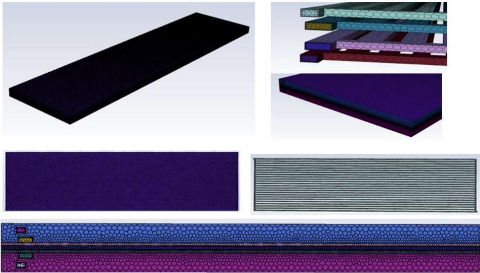
Figure 3: Grid model of the hydrogen fuel cell with parallel reactant flow channels.
