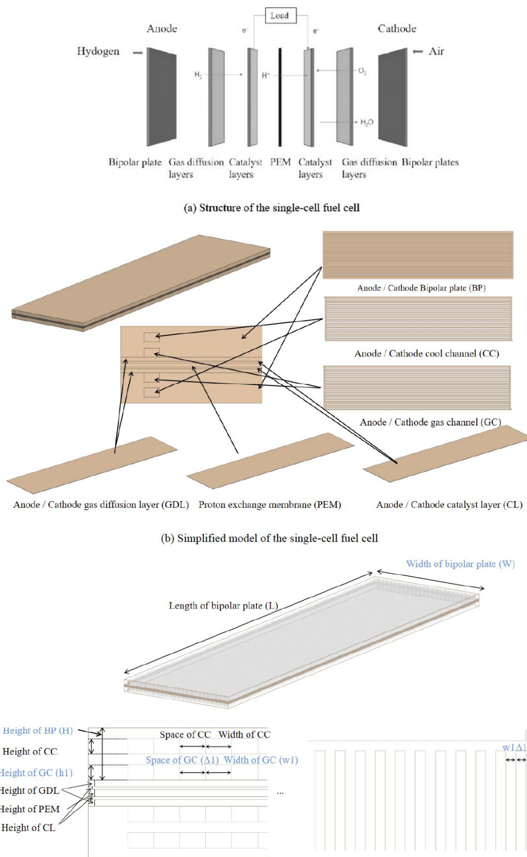
(c) Schematic diagram of the single-cell structural parameters
